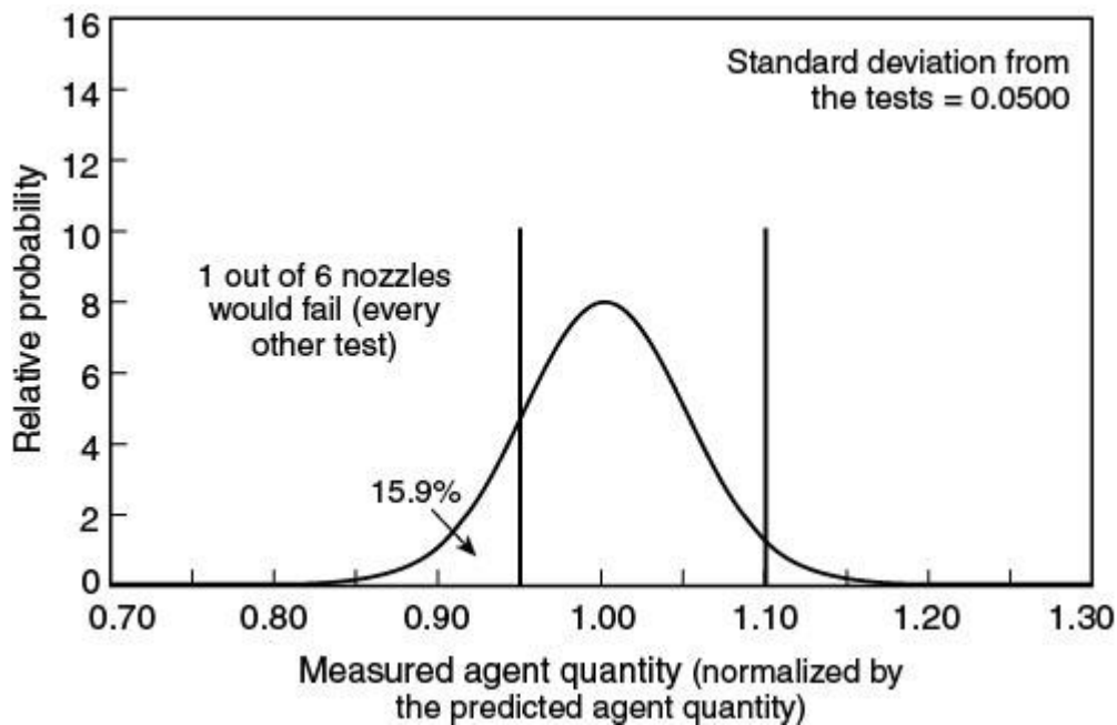
Figure A.7.3.3.2(g) Distribution Curve No. 6.
