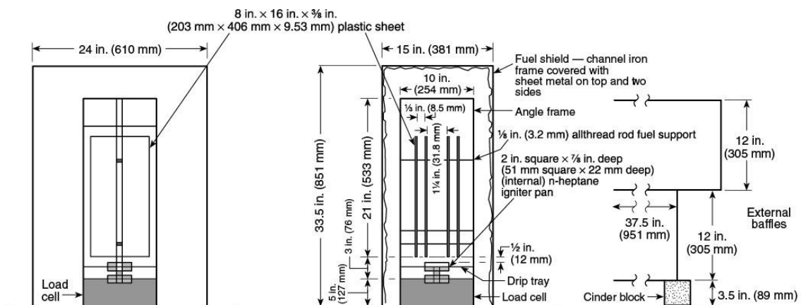
Figure A.7.2.2.3(a) Four-Piece Modified Plastic Setup.
