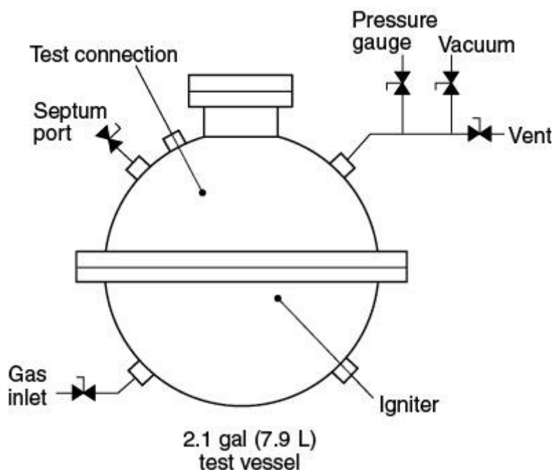
Figure A.7.2.3.1 Spherical Test Vessel.
