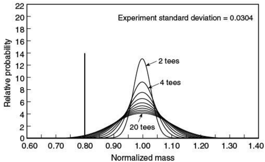
Figure A.7.3.3.2(c) Distribution Curve No. 2.
