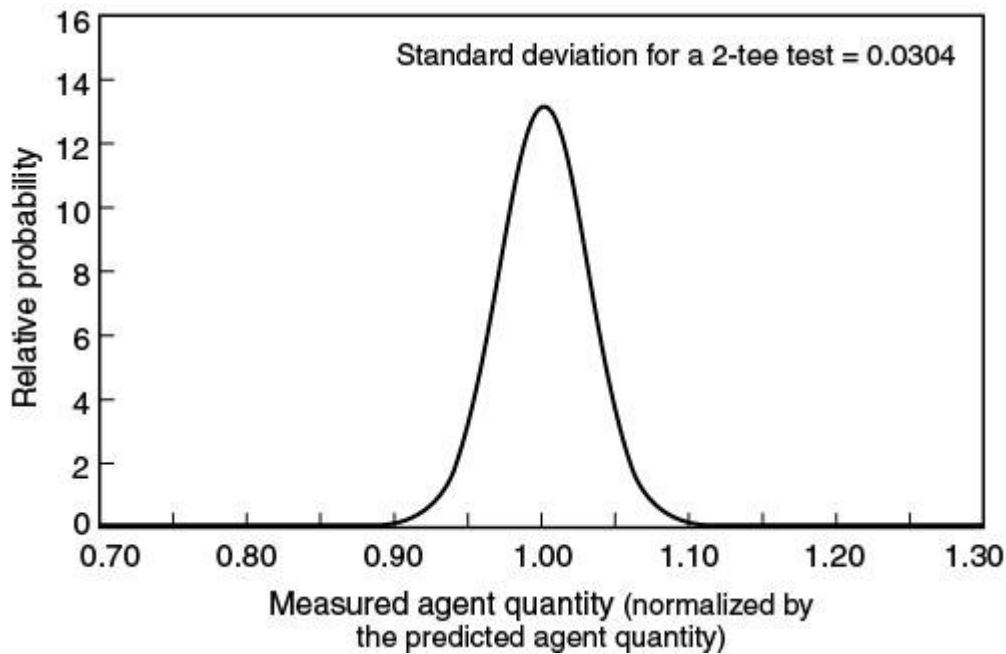
Figure A.7.3.3.2(a) Normal Distribution Curve.
