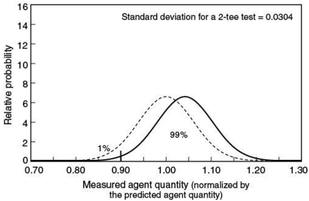
Figure A.7.3.3.2(d) Distribution Curve No. 3.
