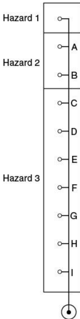
Figure A.7.3.3.1(a) Piping for Design Factor Tee Count for Example 1.
