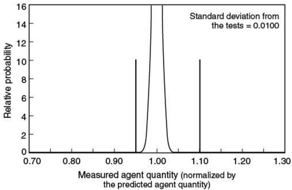
Figure A.7.3.3.2(e) Distribution Curve No. 4.
