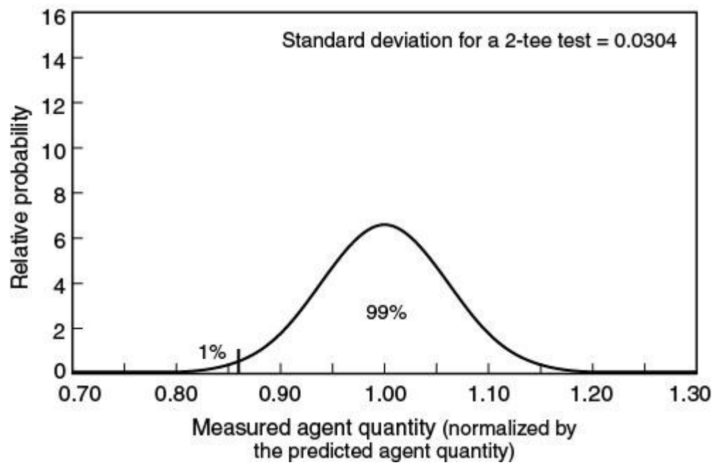
Figure A.7.3.3.2(b) Distribution Curve No. 1.
