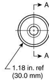
Figure C.17(c) Cup Material: Quartz [Dimensions in Inches (Millimeters)].
