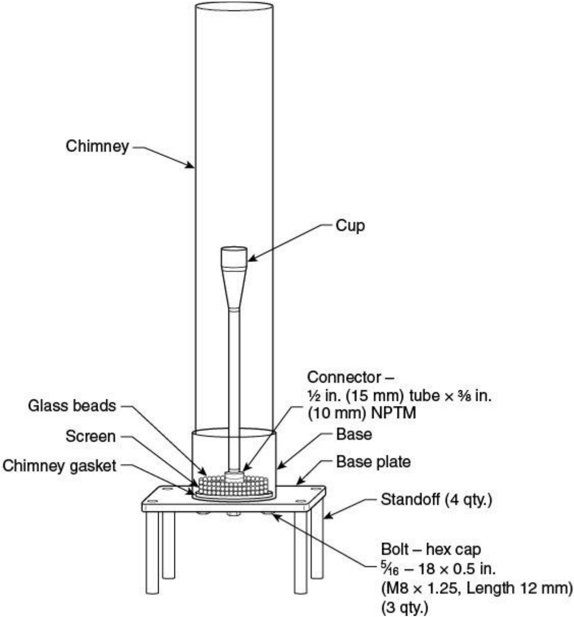
Figure C.17(b) Cup Burner Assembly (Transparent View).
