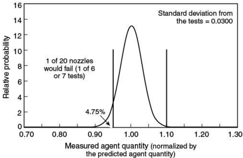
Figure A.7.3.3.2(f) Distribution Curve No. 5.
