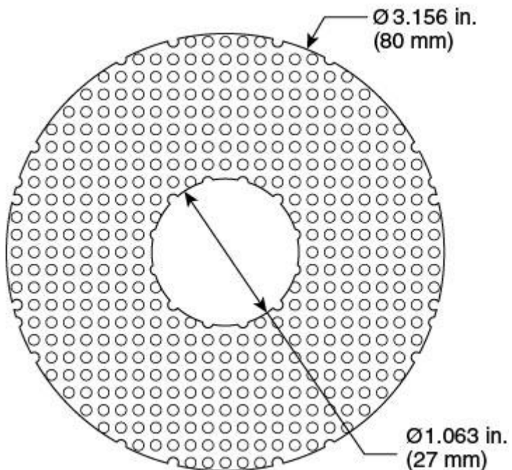
Figure C.17(f) Diffuser Bead Support Screen. (Material: 304 SS).
