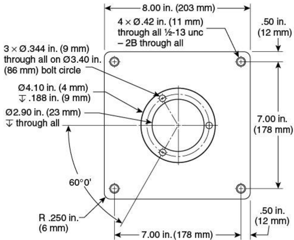
Figure C.17(e) Base Support Plate, 3/8 in. (10 mm) Thick.
