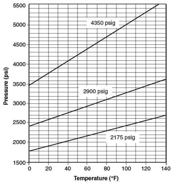
Figure A.5.1.4.1(l) Isometric Diagram of IG-55 Filled at 59°F (15°C).
