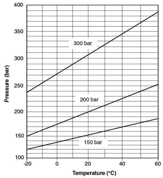
Figure A.5.1.4.1(l) Isometric Diagram of IG-55 Filled at 59°F (15°C).
